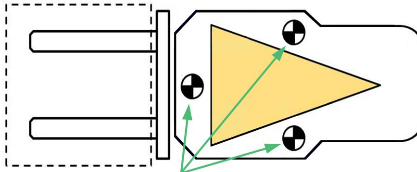
CG - Forklift will tip over
